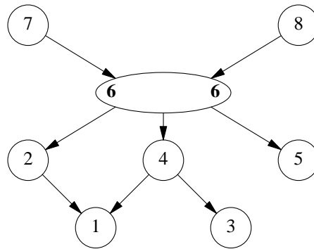
Topological numbering after cycle collapsing.
